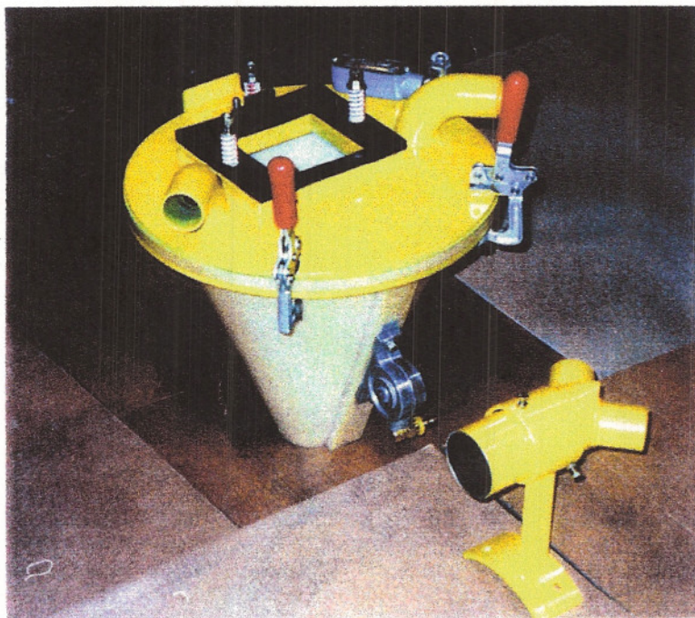
COMPLETELY PRE-ASSEMBLED FOR RETRO-FIT.
